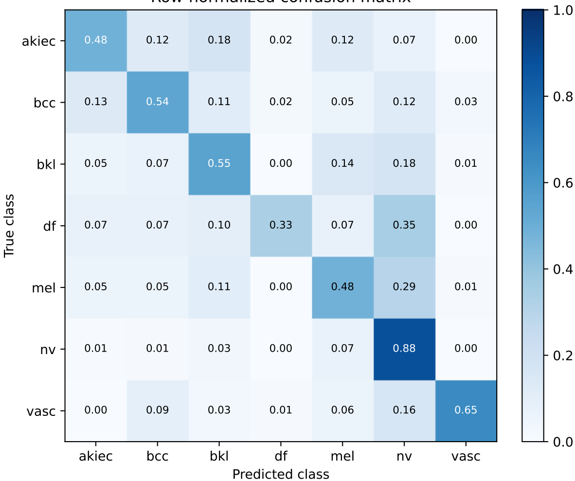
S72 rbf_nystroem | train-only lesion-group OOF Row-normalized confusion matrix
