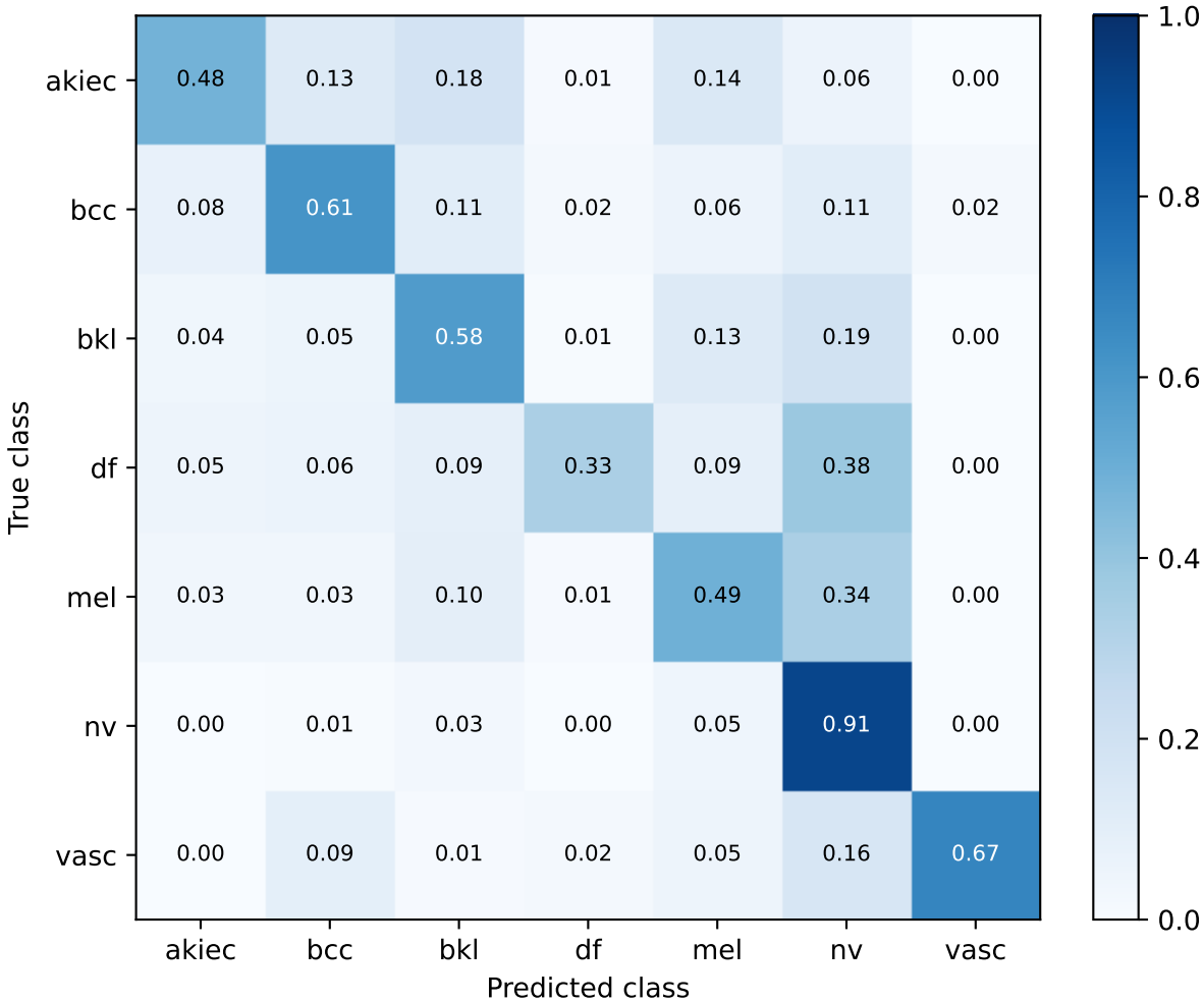
S73 ce_supcon | training-only lesion-group OOF Row-normalized confusion matrix
