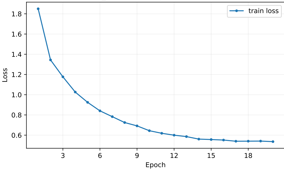
S73 ce_supcon fold2 | CPU head training
