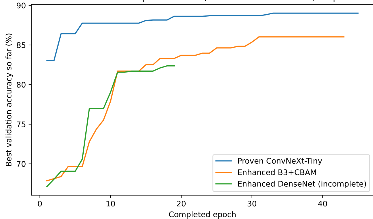
Same strict development cohort; different architectures/recipes
