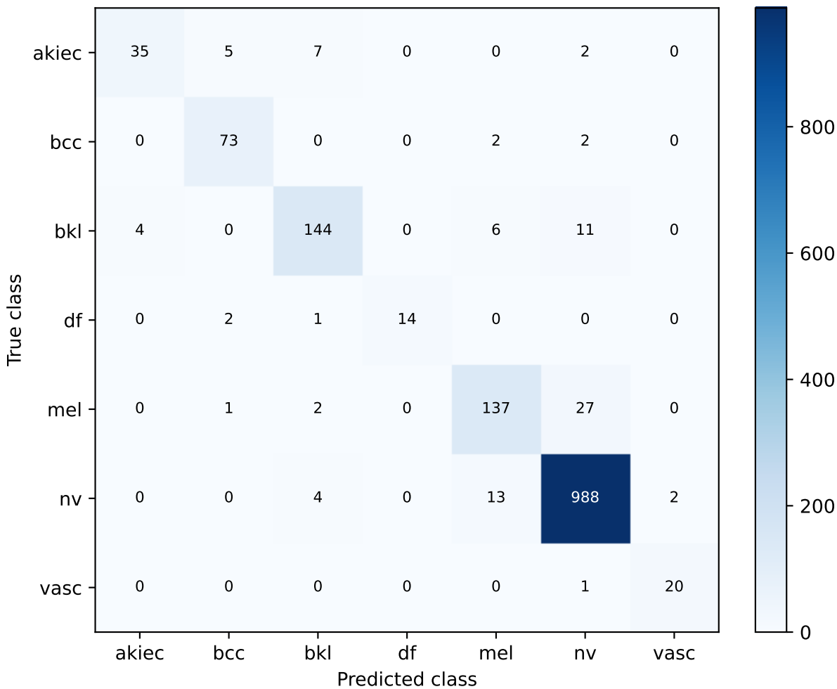
S84 cbam_only_fixed_temperature | exploratory validation Confusion matrix
