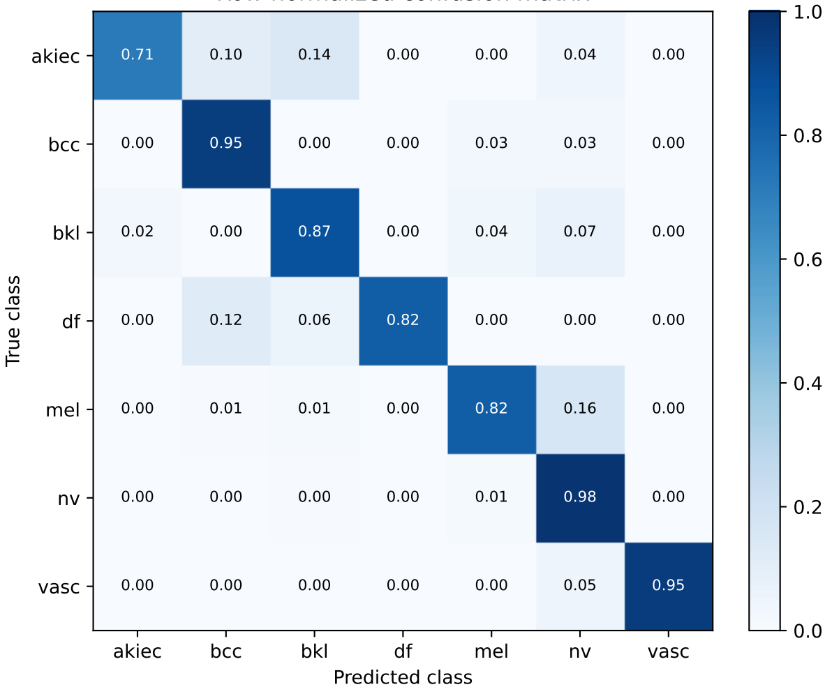
S84 cbam_only_fixed_temperature | exploratory validation Row-normalized confusion matrix
