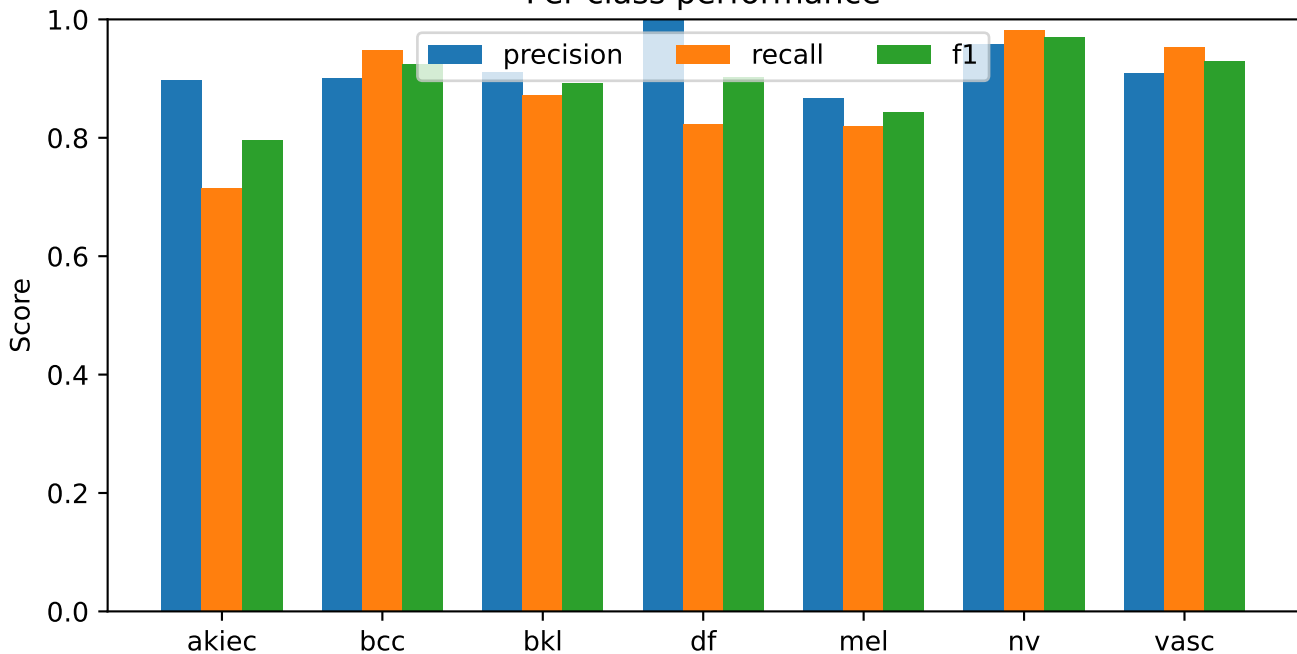
S84 cbam_only_fixed_temperature | exploratory validation Per-class performance
