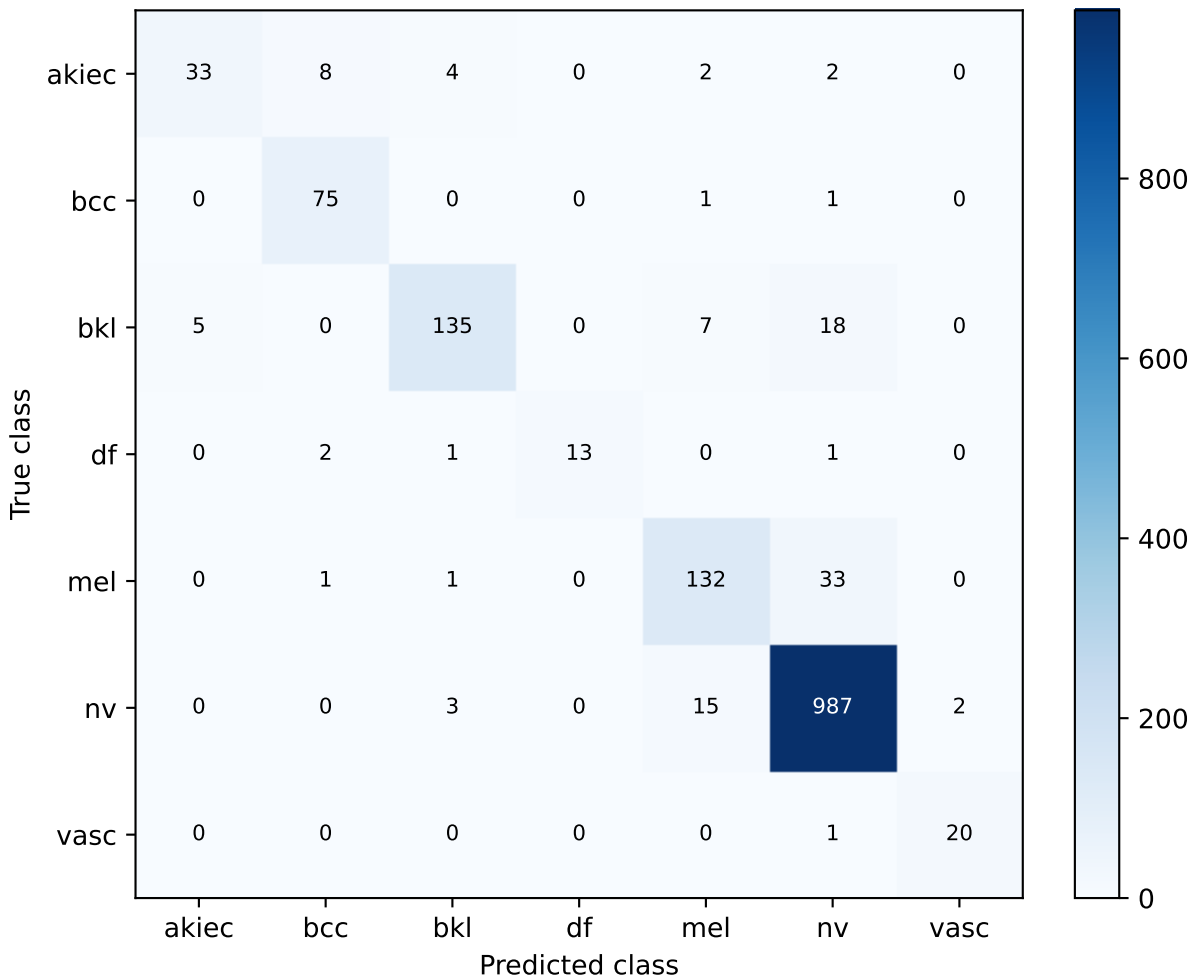
S45 equal_geometric_fusion | exploratory validation Confusion matrix
