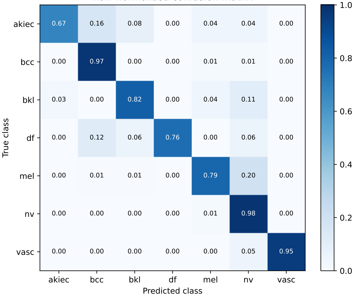
S45 equal_geometric_fusion | exploratory validation Row-normalized confusion matrix
