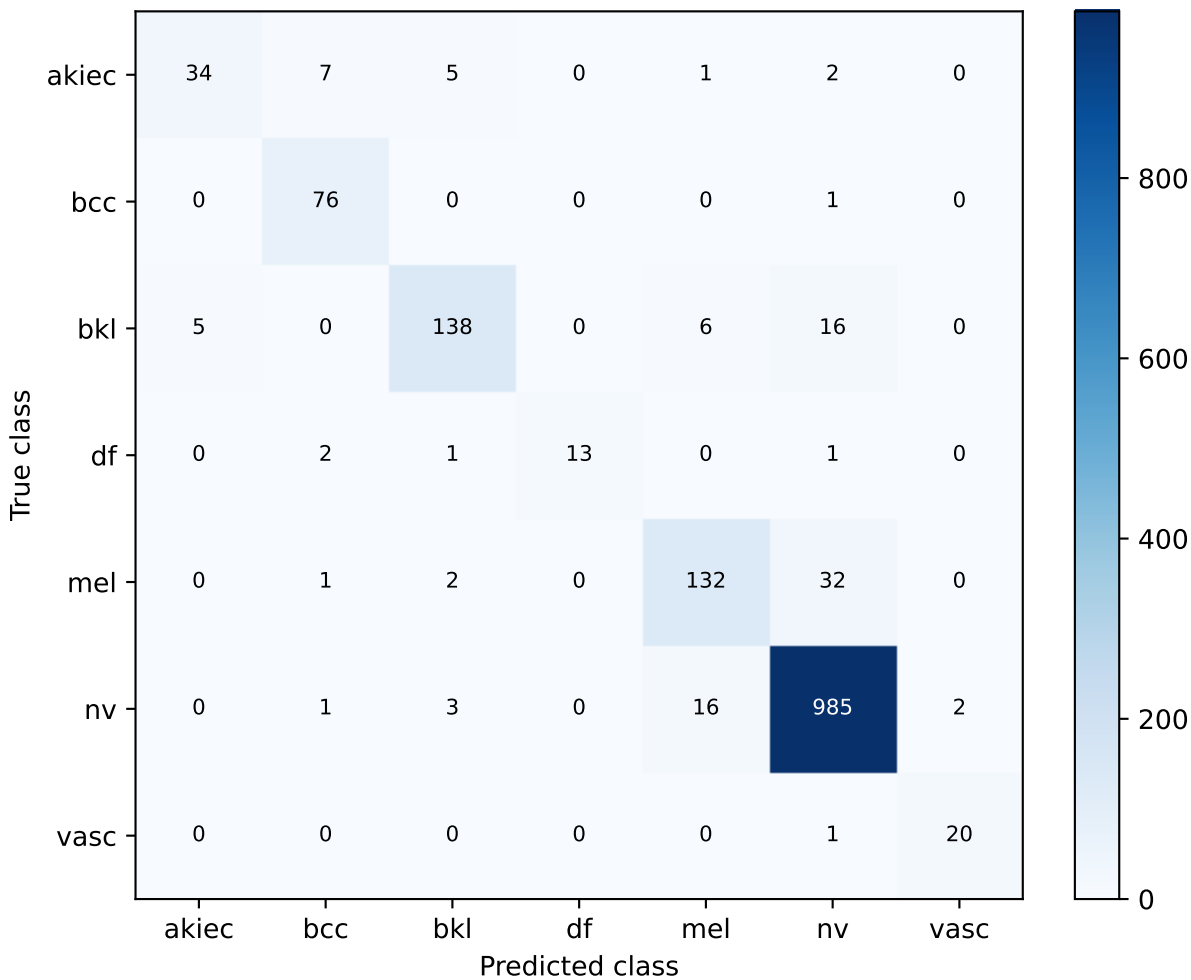
S43 strong_convnext_weights | exploratory validation Confusion matrix
