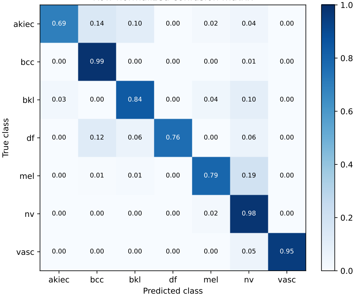
S43 strong_convnext_weights | exploratory validation Row-normalized confusion matrix
