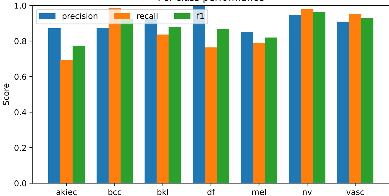
S43 strong_convnext_weights | exploratory validation Per-class performance
