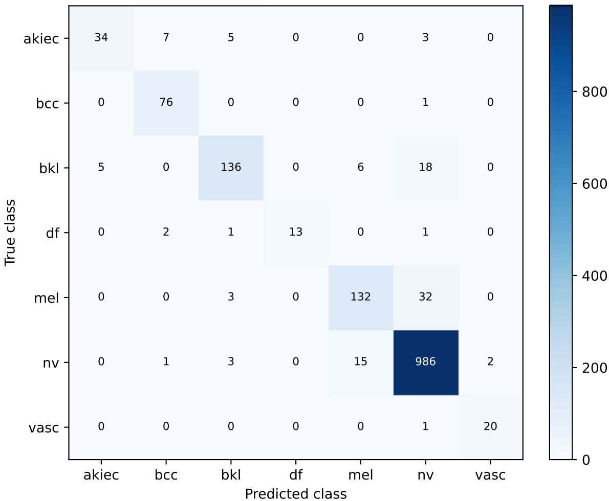
S44 tiny_emphasis_weights | exploratory validation Confusion matrix
