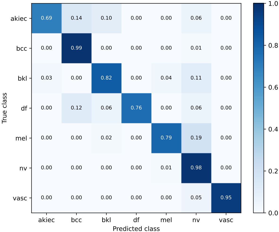
S44 tiny_emphasis_weights | exploratory validation Row-normalized confusion matrix
