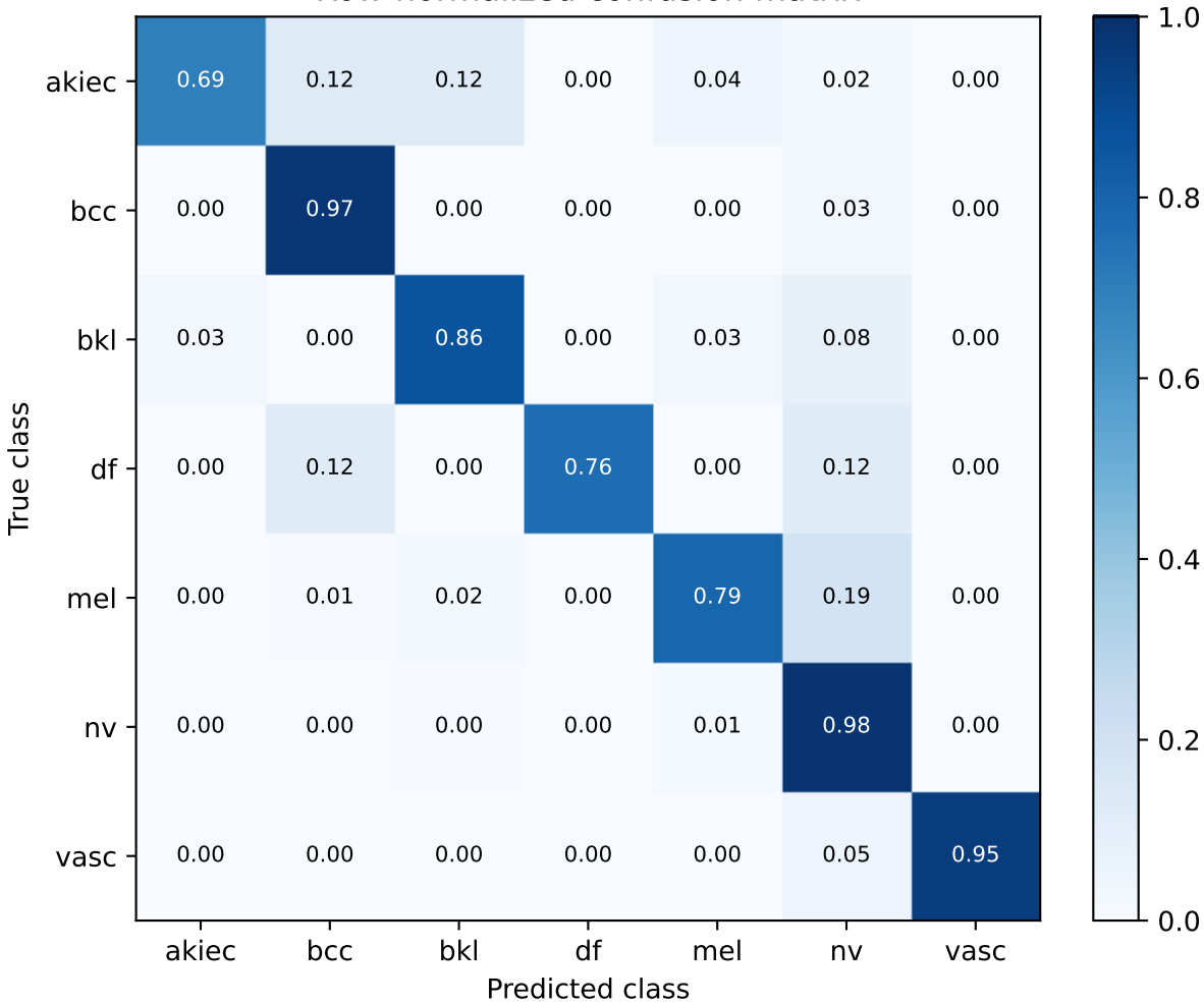
S46 fixed F1 checkpoint rule | exploratory validation Row-normalized confusion matrix
