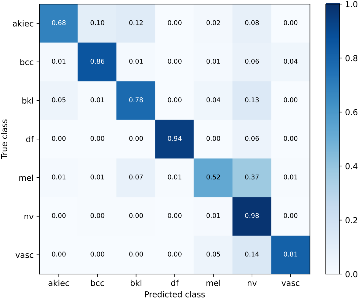
reference_plus_b3_dense_equal | post-test strict development screening Row-normalized confusion matrix
