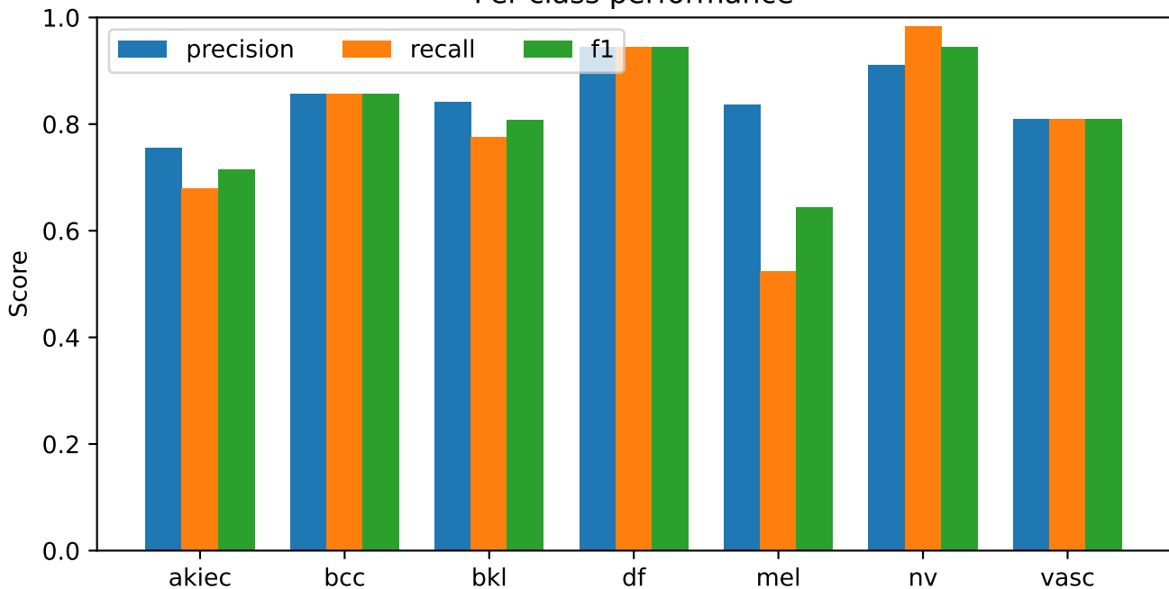
reference_plus_b3_dense_equal | post-test strict development screening Per-class performance
