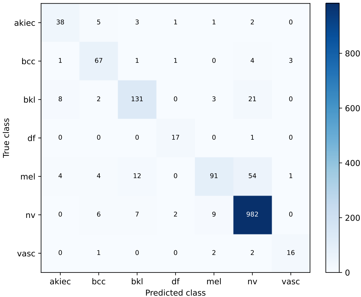
reference_plus_dense_equal | post-test strict development screening Confusion matrix
