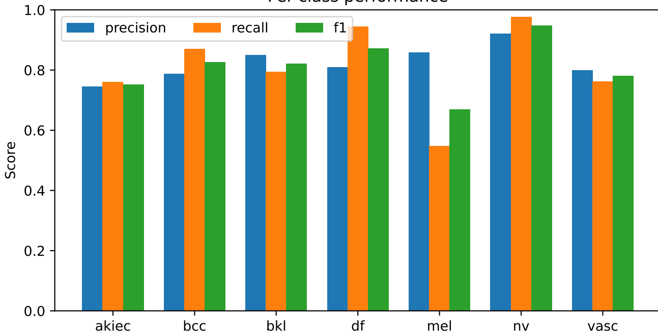
reference_plus_dense_equal | post-test strict development screening Per-class performance
