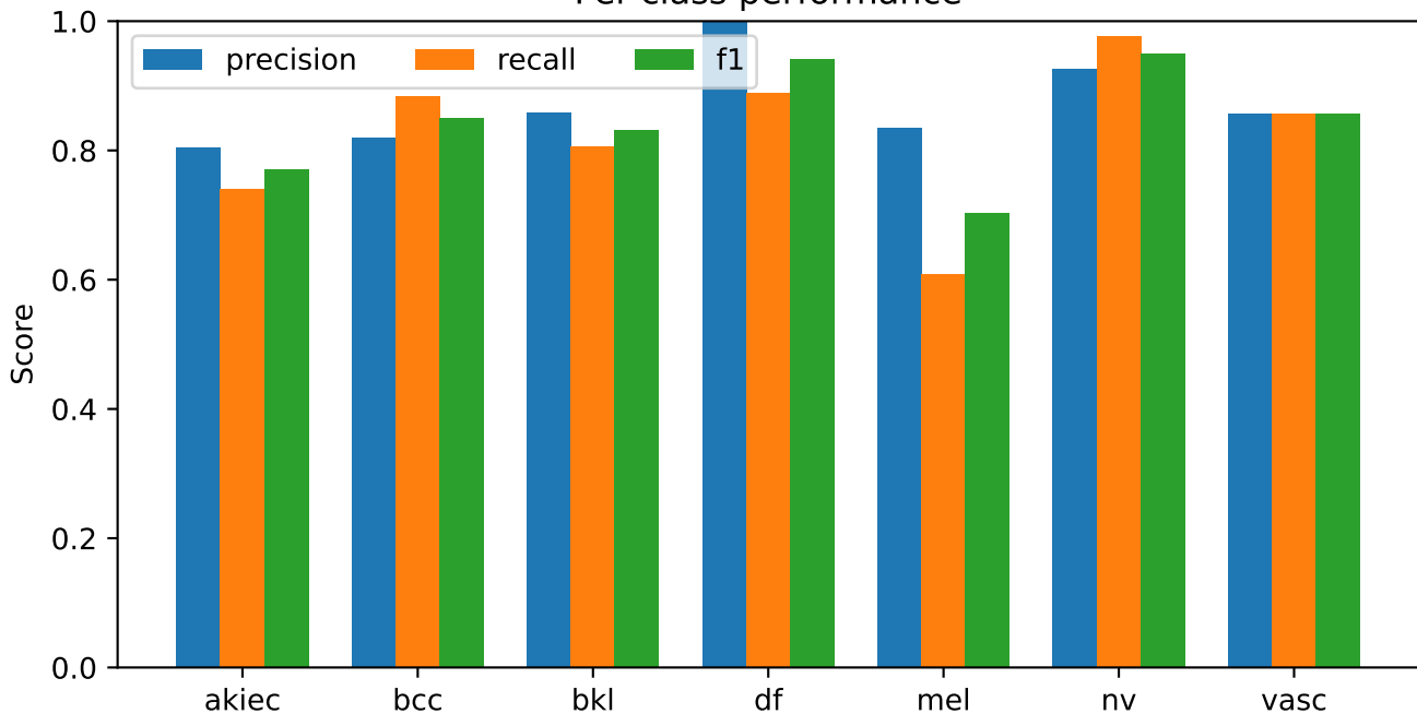
strict_reference | post-test strict development screening Per-class performance
