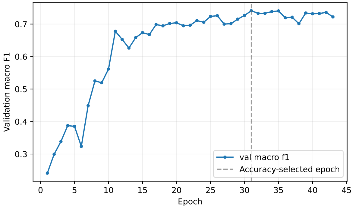
efficientnet_b3 | enhanced development
