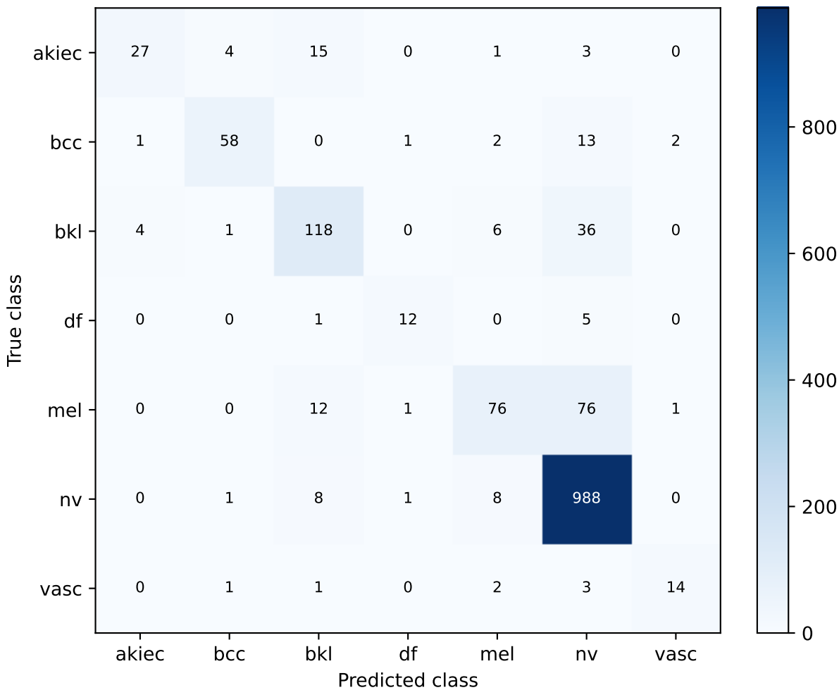
efficientnet_b3 | enhanced lesion-disjoint validation Confusion matrix
