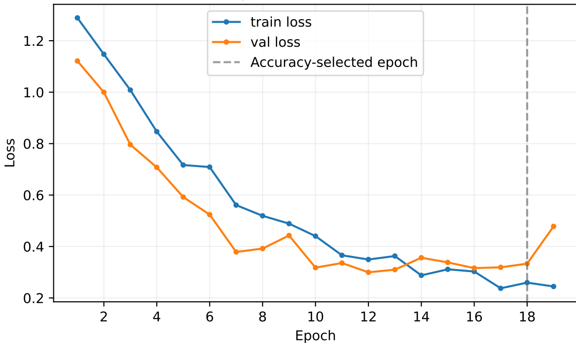
DenseNet201 | incomplete budget-stopped run
