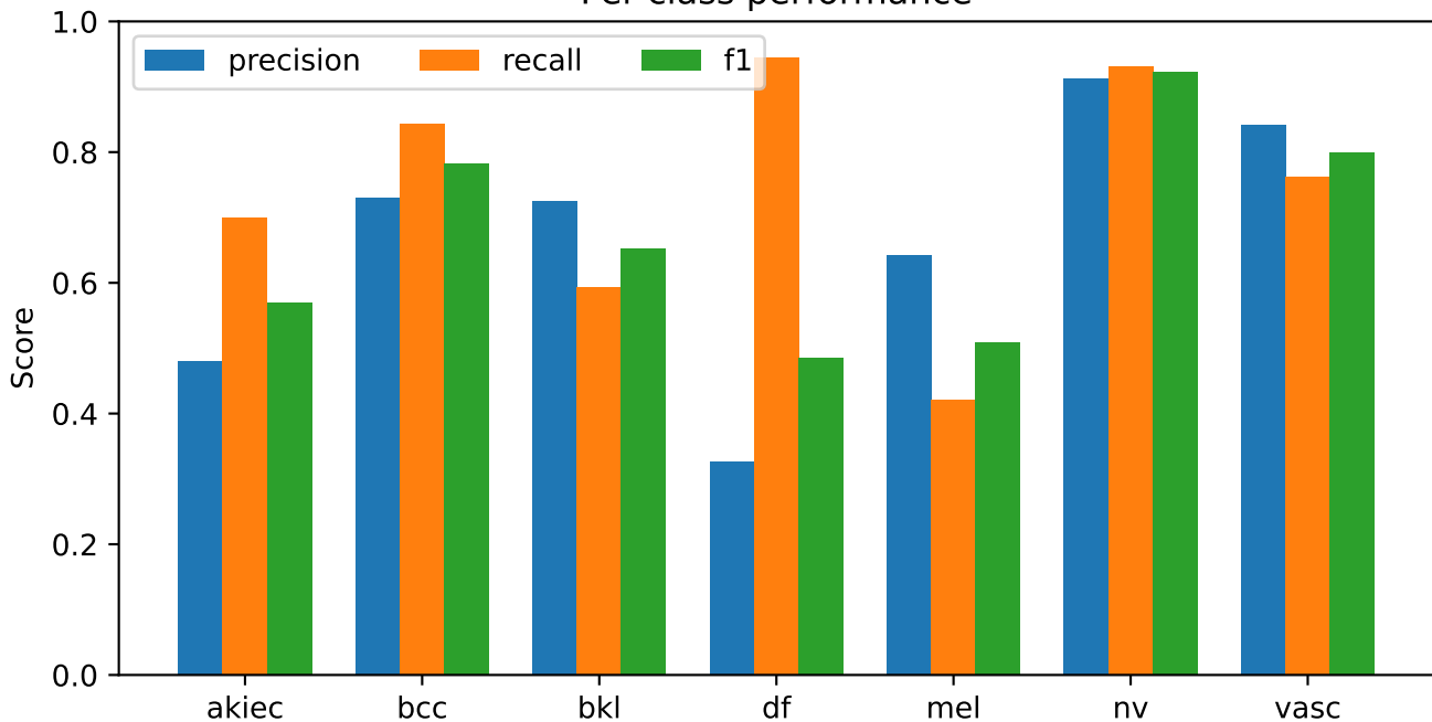
DenseNet201 | budget-stopped development validation Per-class performance
