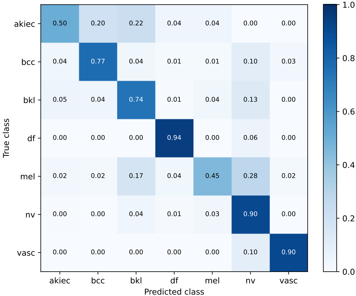
DenseNet201 | budget-stopped development validation Row-normalized confusion matrix
