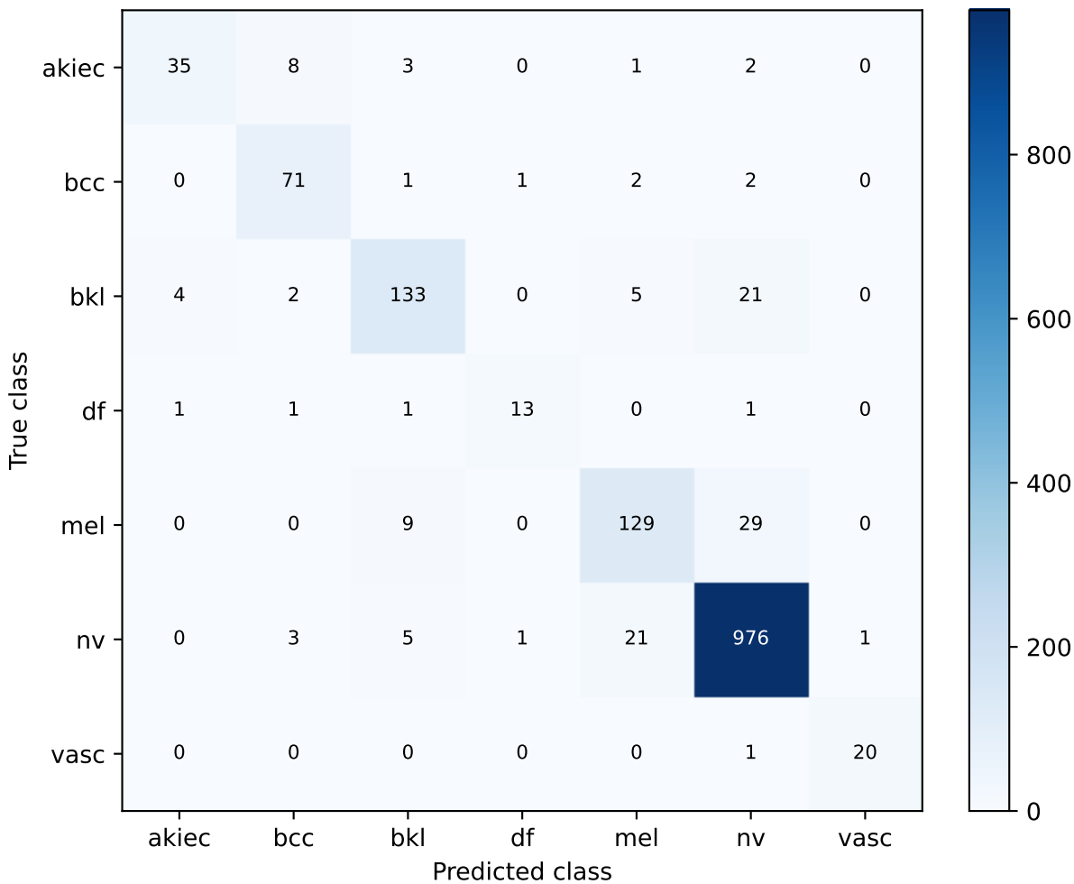
S95 ConvNeXt-Tiny decay0.05 | exploratory validation Confusion matrix
