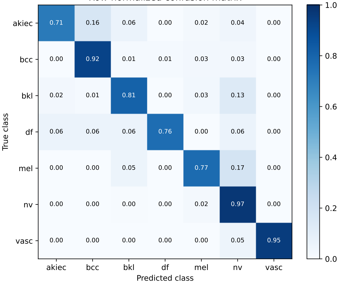
S95 ConvNeXt-Tiny decay0.05 | exploratory validation Row-normalized confusion matrix
