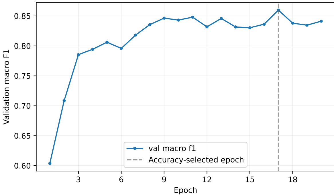
S95 ConvNeXt-Tiny decay0.05 training
