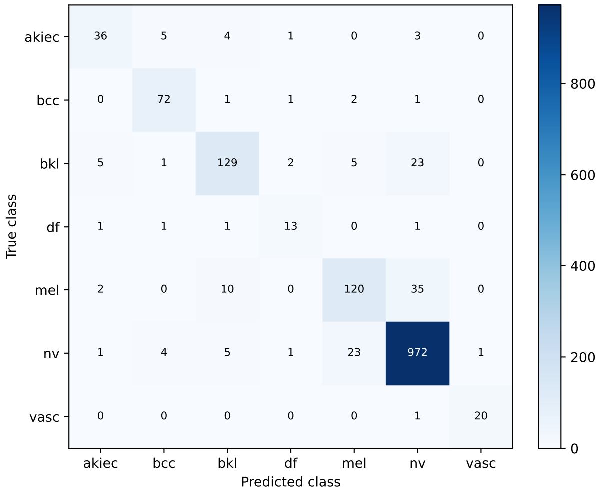
S95 ConvNeXt-Tiny decay0.05 final committed epoch | exploratory validation Confusion matrix
