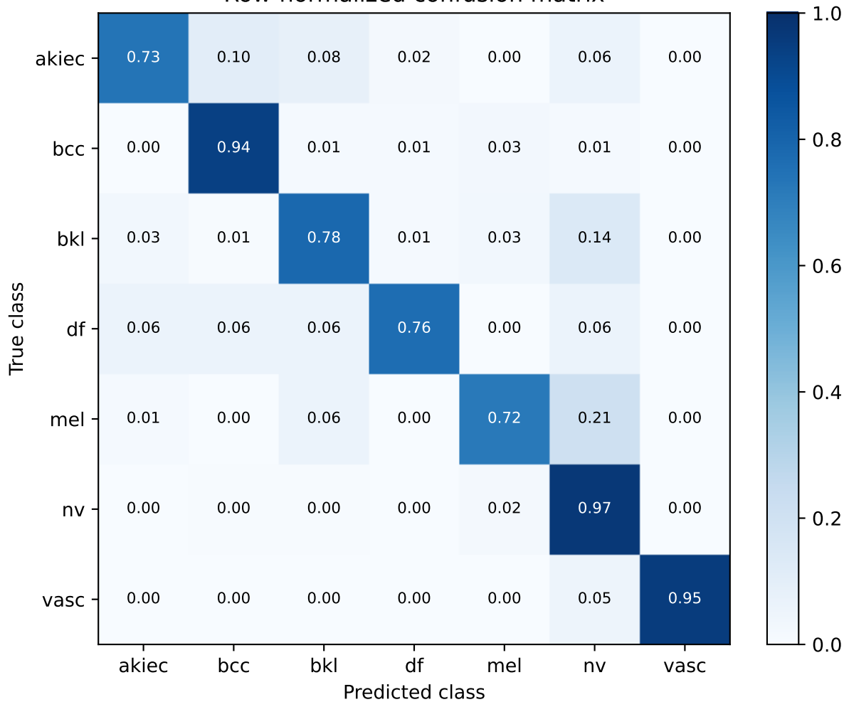
S95 ConvNeXt-Tiny decay0.05 final committed epoch | exploratory validation Row-normalized confusion matrix
