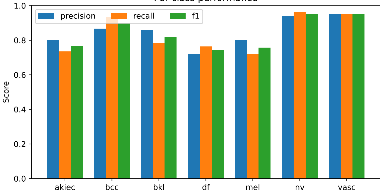
S95 ConvNeXt-Tiny decay0.05 final committed epoch | exploratory validation Per-class performance
