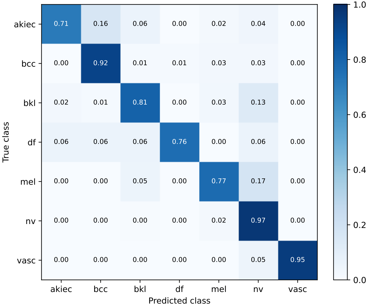
S95 ConvNeXt-Tiny decay0.05 | exploratory validation_macro_f1 Row-normalized confusion matrix
