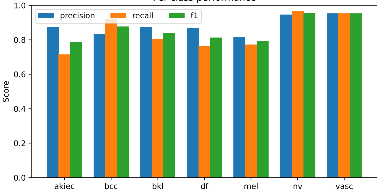
S95 ConvNeXt-Tiny decay0.05 | exploratory validation_macro_f1 Per-class performance
