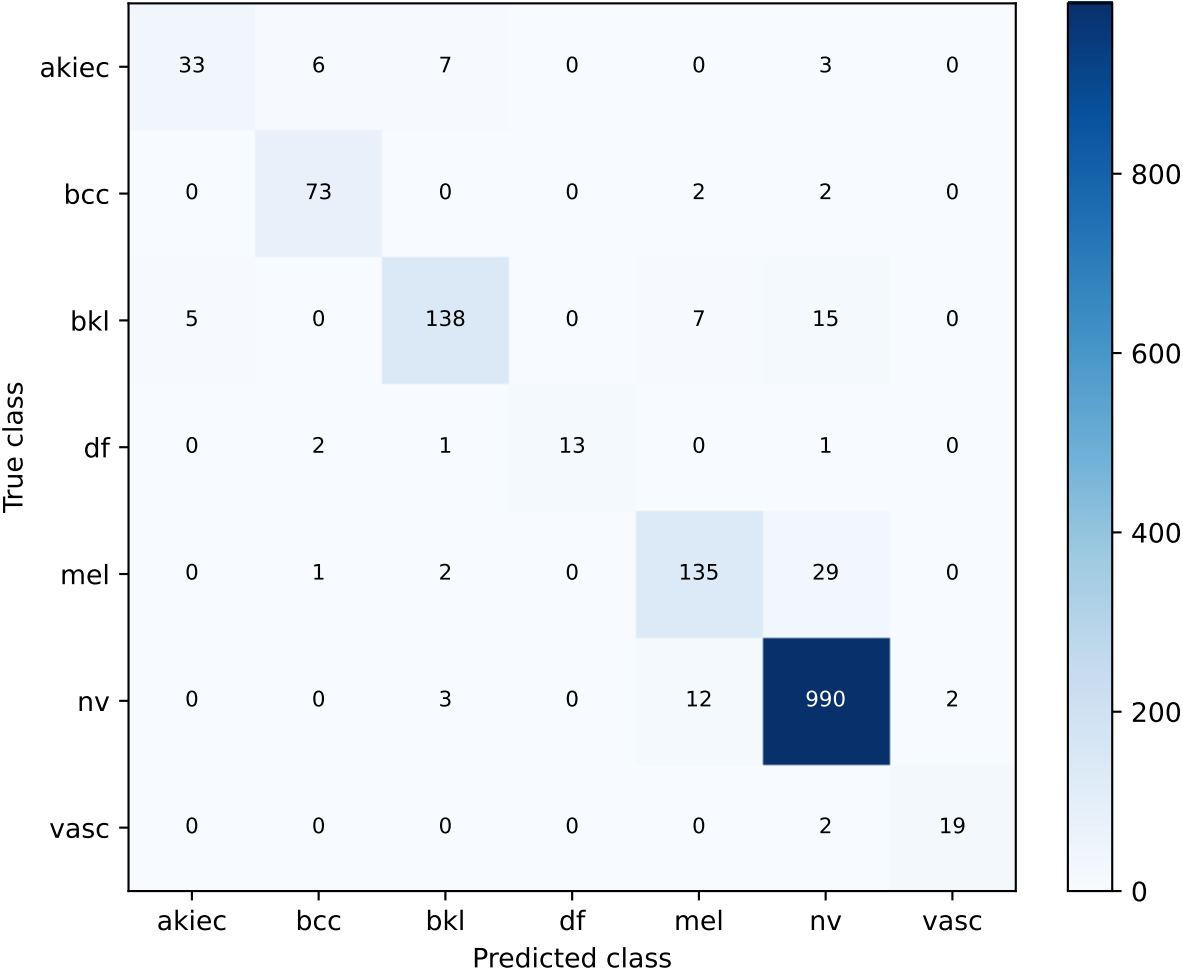
S96 fixed stronger-decay Tiny replacement | exploratory validation Confusion matrix
