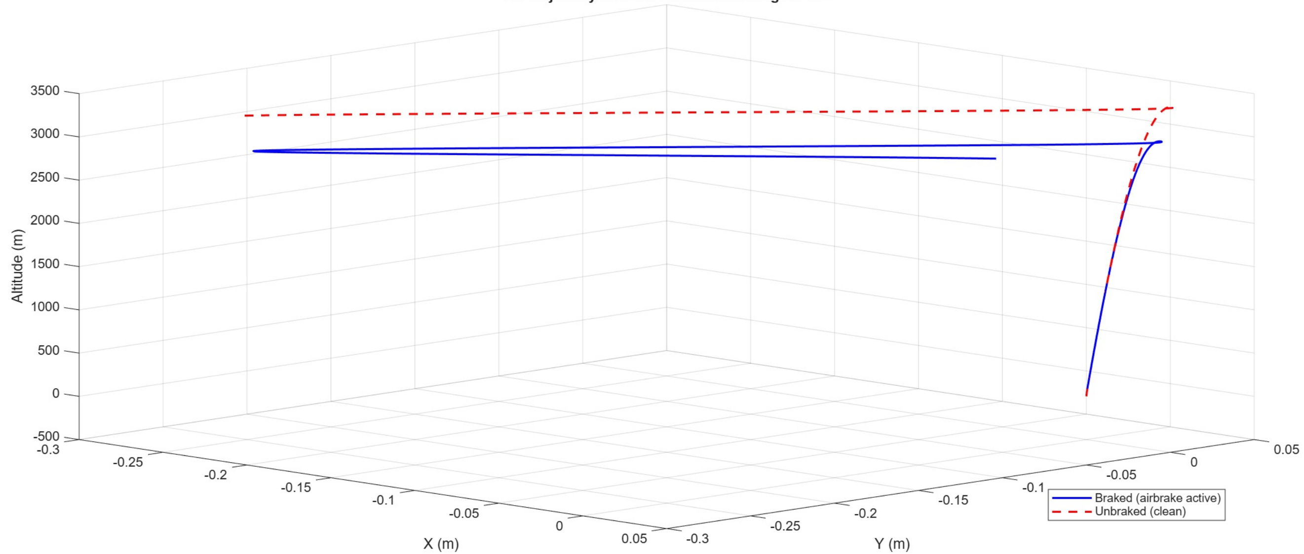
3D Trajectory: Braked vs. Unbraked Flight Path
