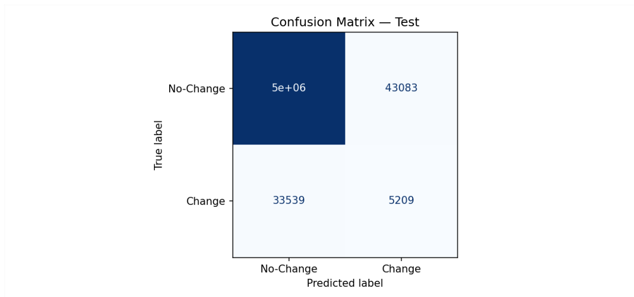
Figure 4: Confusion matrix on the test split. The higher false positive and false negative counts relative to true positives reflect the generalisation gap from limited training data.
