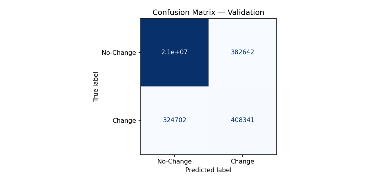
Figure 3: Confusion matrix on the validation split. Rows = actual class, Columns = predicted class.
