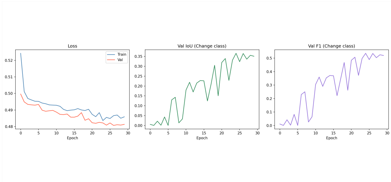
Figure 2: Training curves over 30 epochs. Left: train and validation loss. Centre: validation IoU (Change class). Right: validation F1 (Change class). Best checkpoint at epoch 25.
