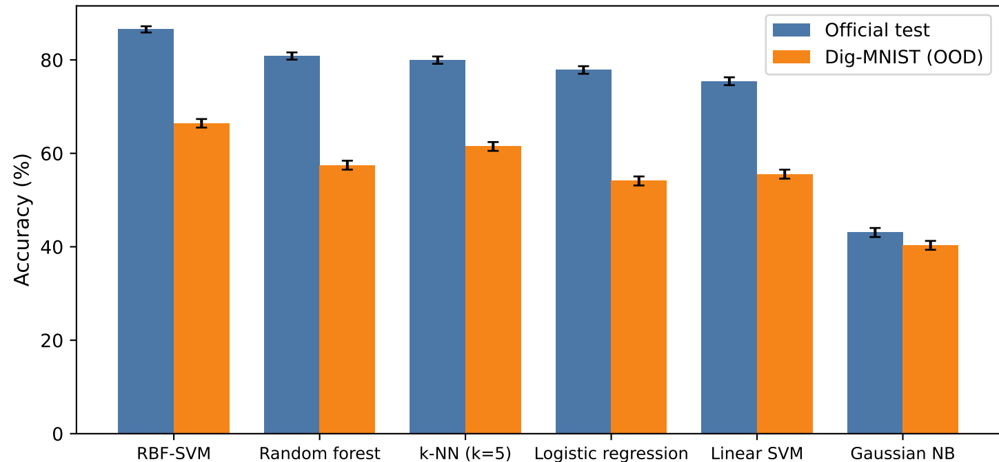
Classifier comparison on KTSD features (official 60k training, 95% Wilson intervals)
