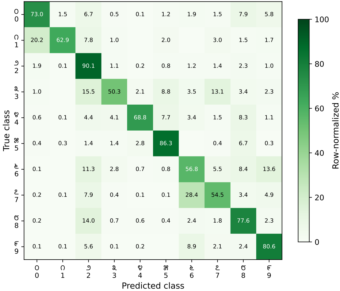
KTSD confusion matrix, Dig-MNIST (out-of-distribution) — accuracy 70.11%
