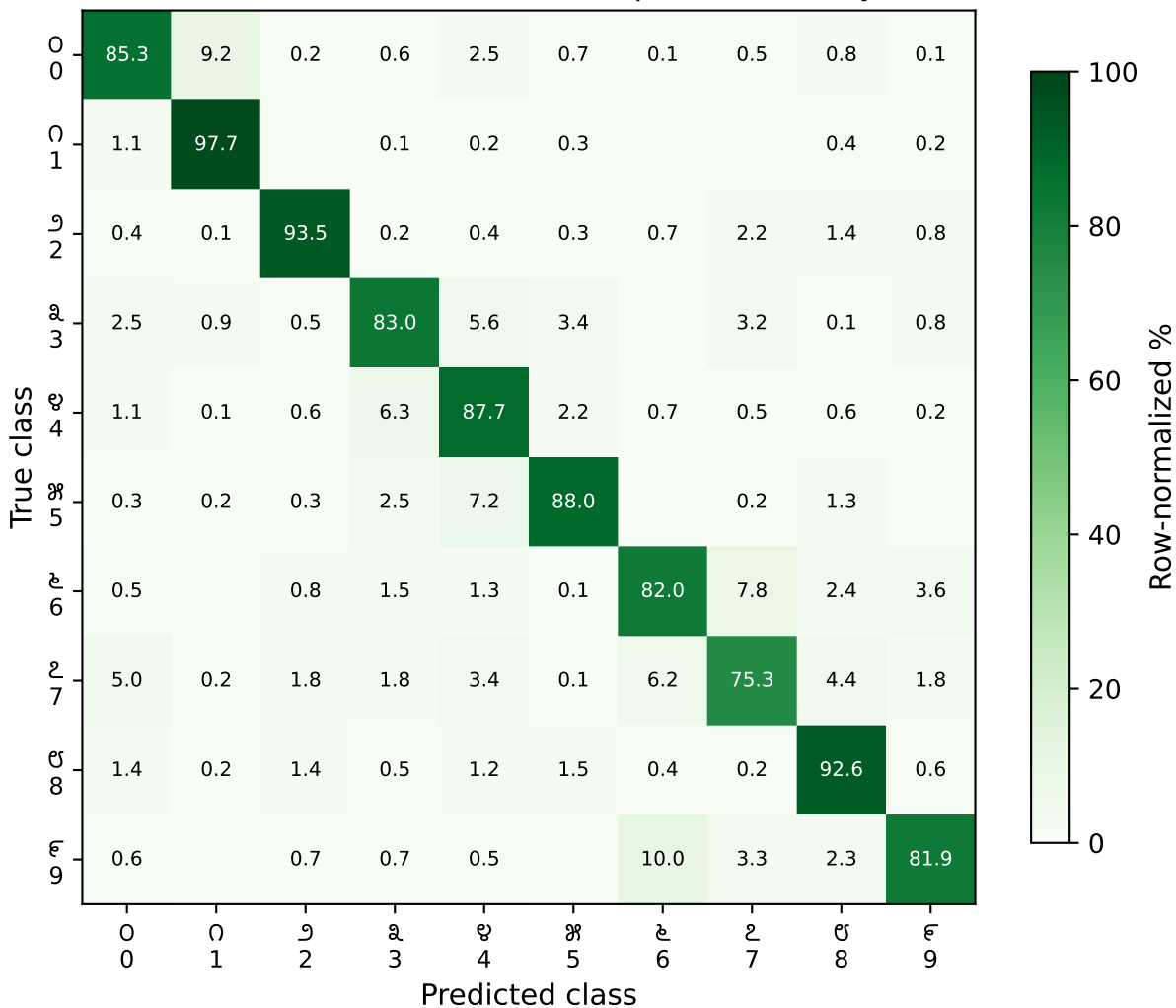
KTSD confusion matrix, Official test split — accuracy 86.70%
