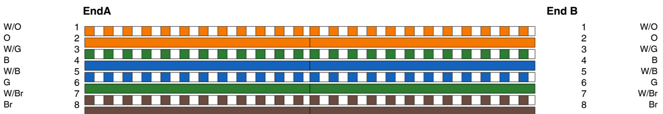
Cable 1: Straight-through cable (T568B - T568B)
