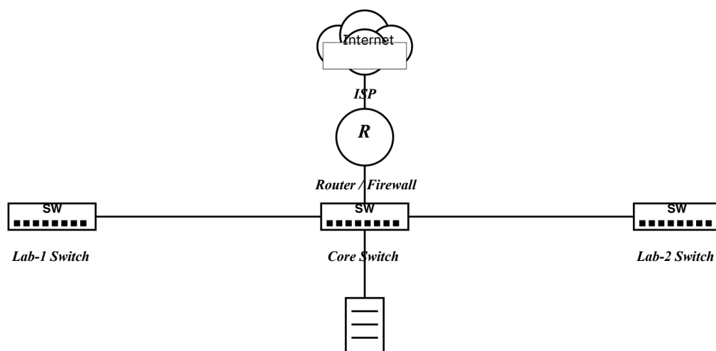
Fig 4: Topology of the college network
