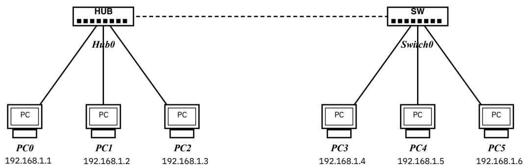
Fig 3: Network using both HUB and SWITCH (6 hosts)
