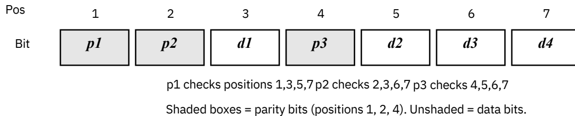
Fig 1: Hamming (7,4) codeword layout
