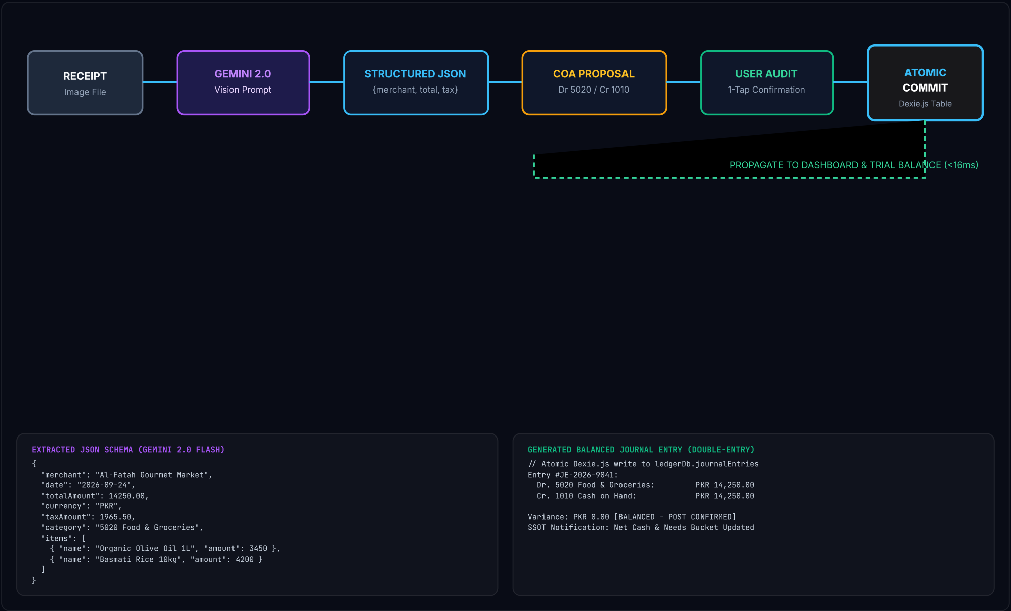
FIG. 08 – OCR TO DOUBLE-ENTRY TRANSACTION PIPELINE From Physical Receipt Pixels to Balanced Double-Entry Journal Entry
