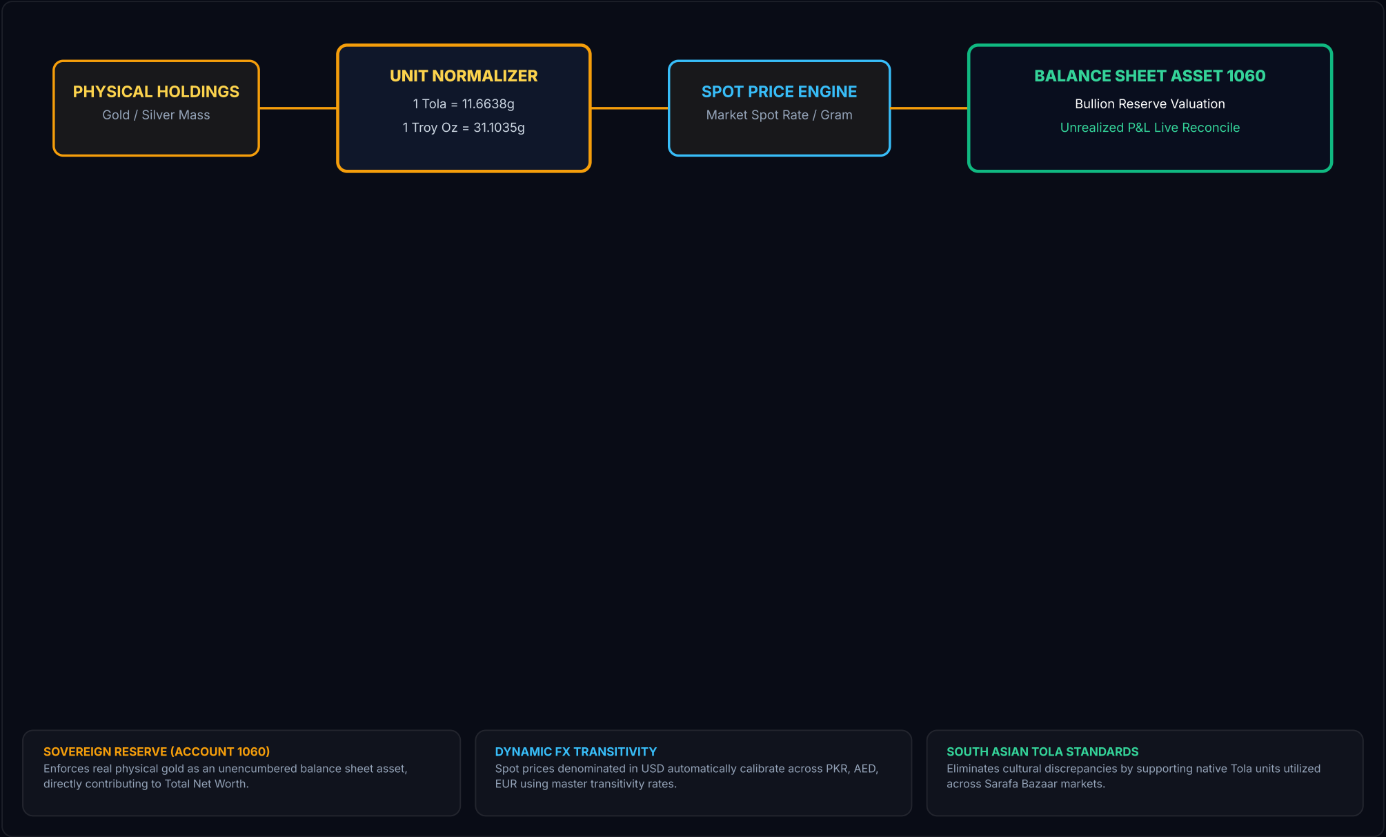
FIG. 15 – BULLION VALUATION & UNIT CONVERSION PIPELINE Grams, Troy Ounces, and South Asian Tola Calculations
