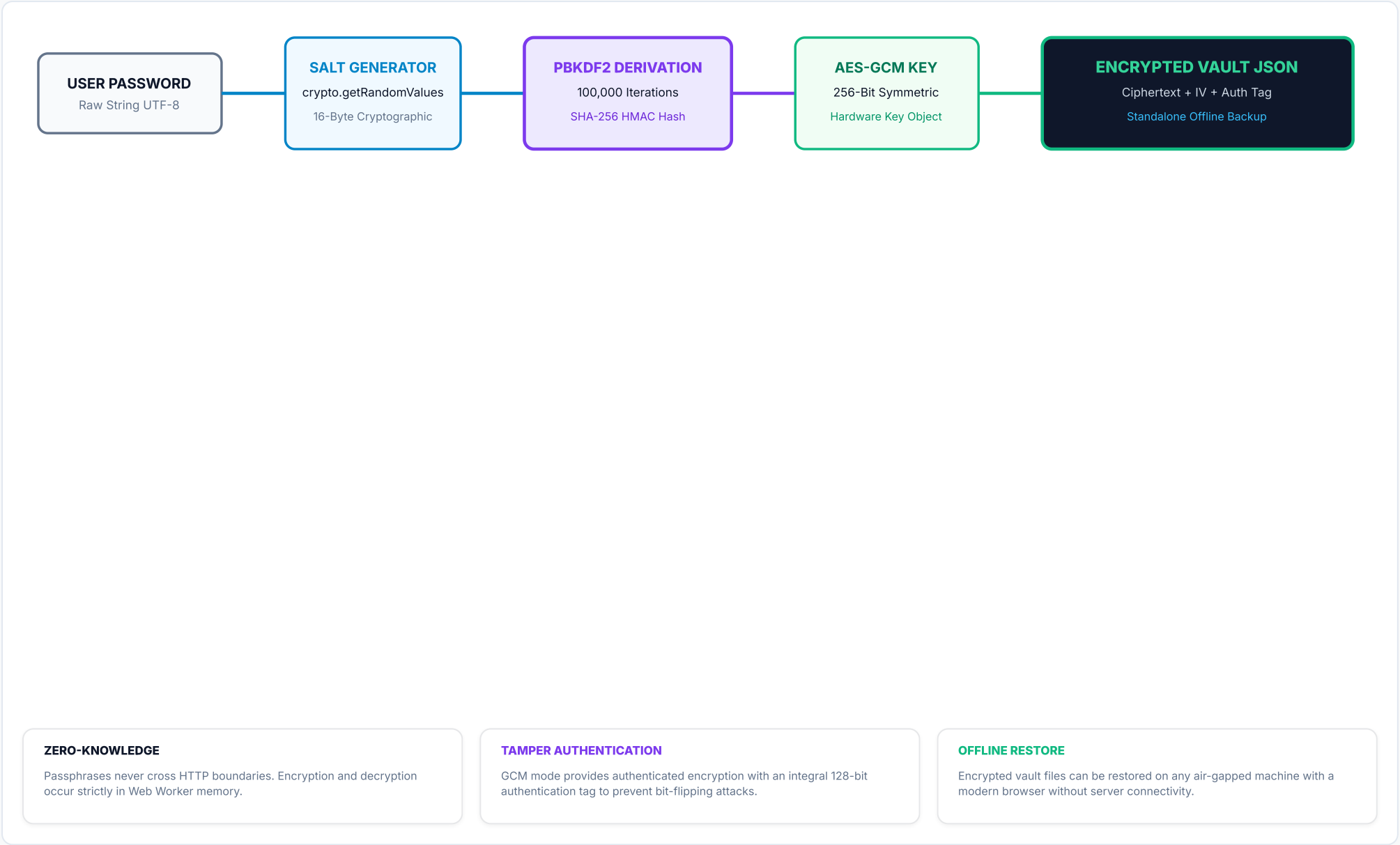
FIG. 12 – VAULT ENCRYPTION & DECRYPTION SEQUENCE
