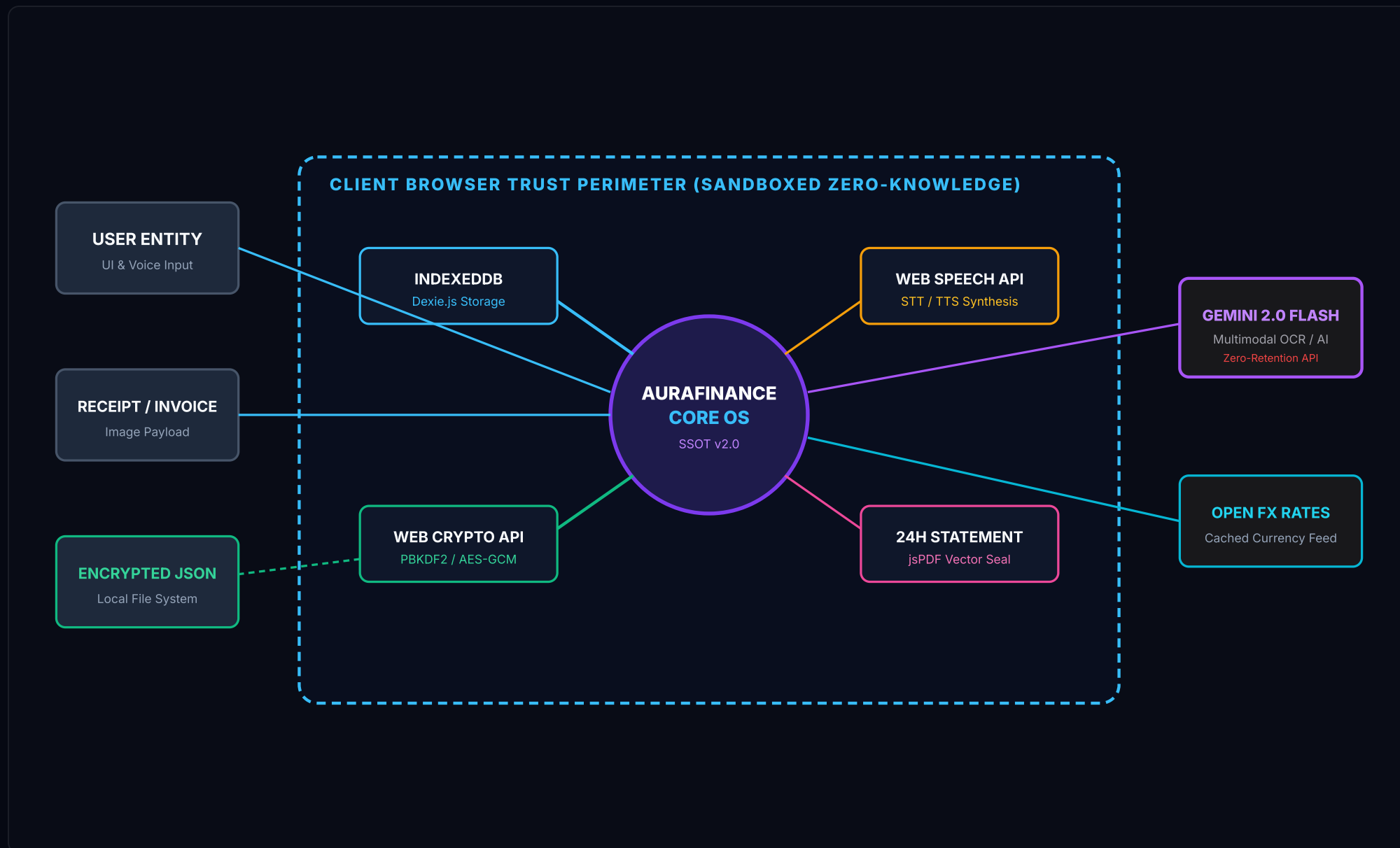
FIG. 01 – LEVEL-0 MACRO CONTEXT DFD
