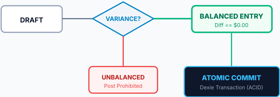
FIG. 04 - DOUBLE-ENTRY COMMIT STATE MACHINE
