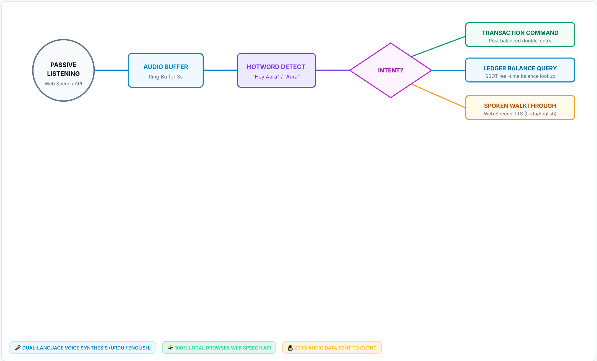
FIG. 09 – VOICE ASSISTANT FINITE STATE MACHINE
