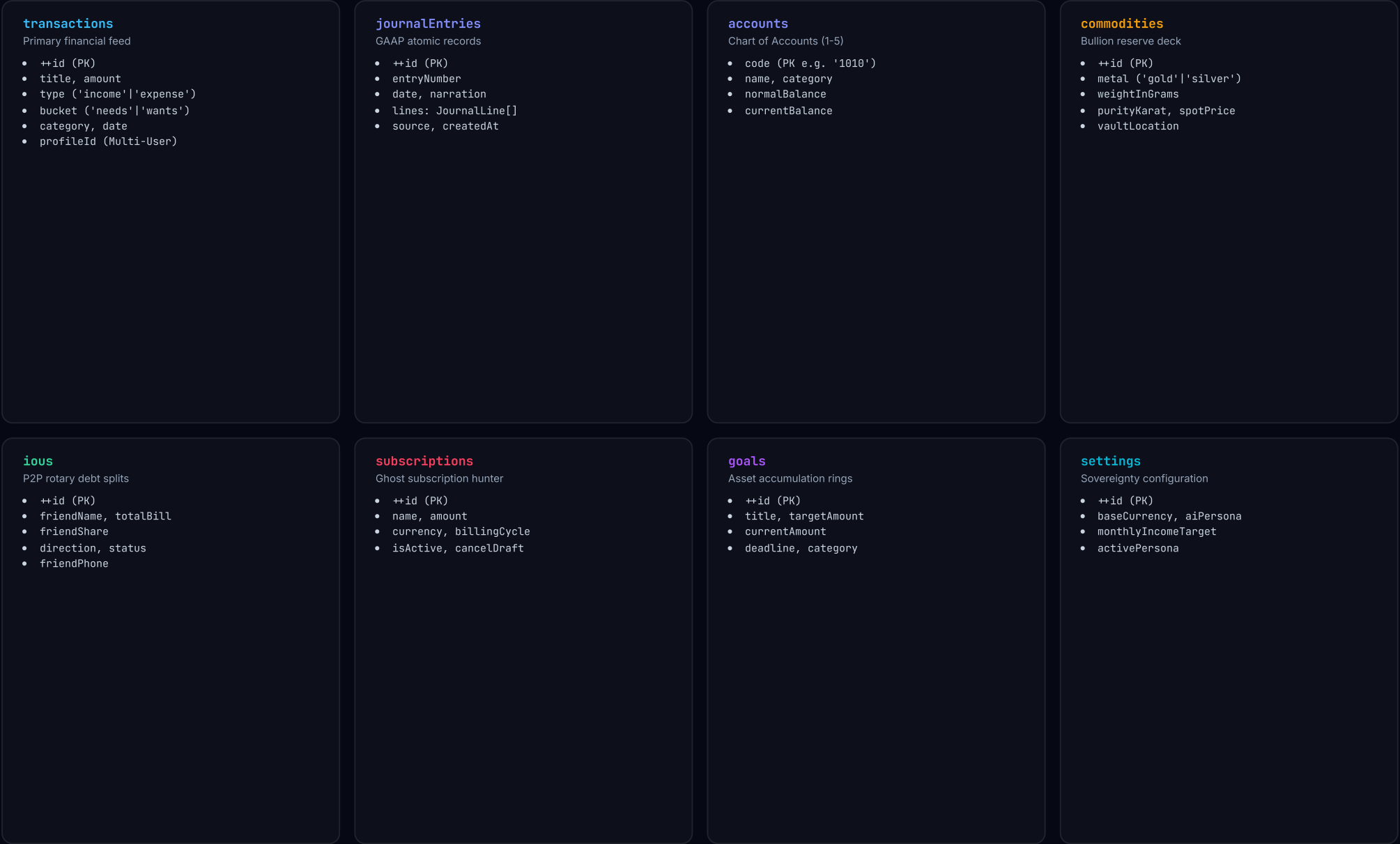
FIG. 13 – DEXIE.JS DATA ENTITY COLLECTIONS
