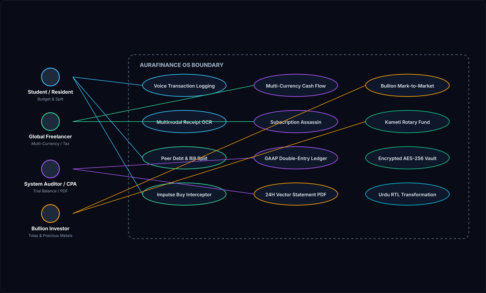
FIG. 06 – COMPREHENSIVE UML USE CASE DIAGRAM Four Specialized Personas Interacting with Autonomous Sub-Systems ACTOR COVERAGE: 100% MODULE CAPABILITIES
