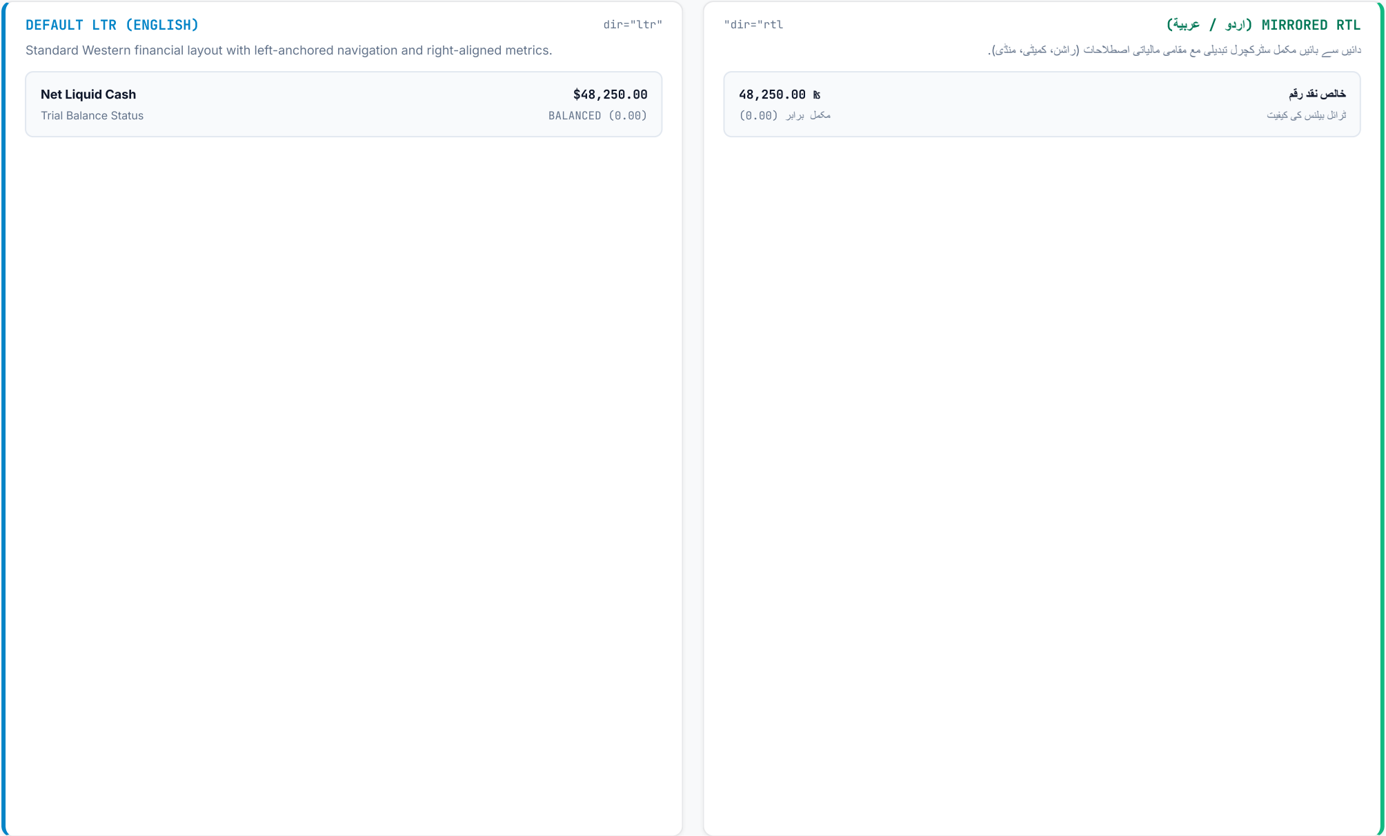
FIG. 17 — DOM DIR="LTR" VS DIR="RTL" MIRRORING ARCHITECTURE
