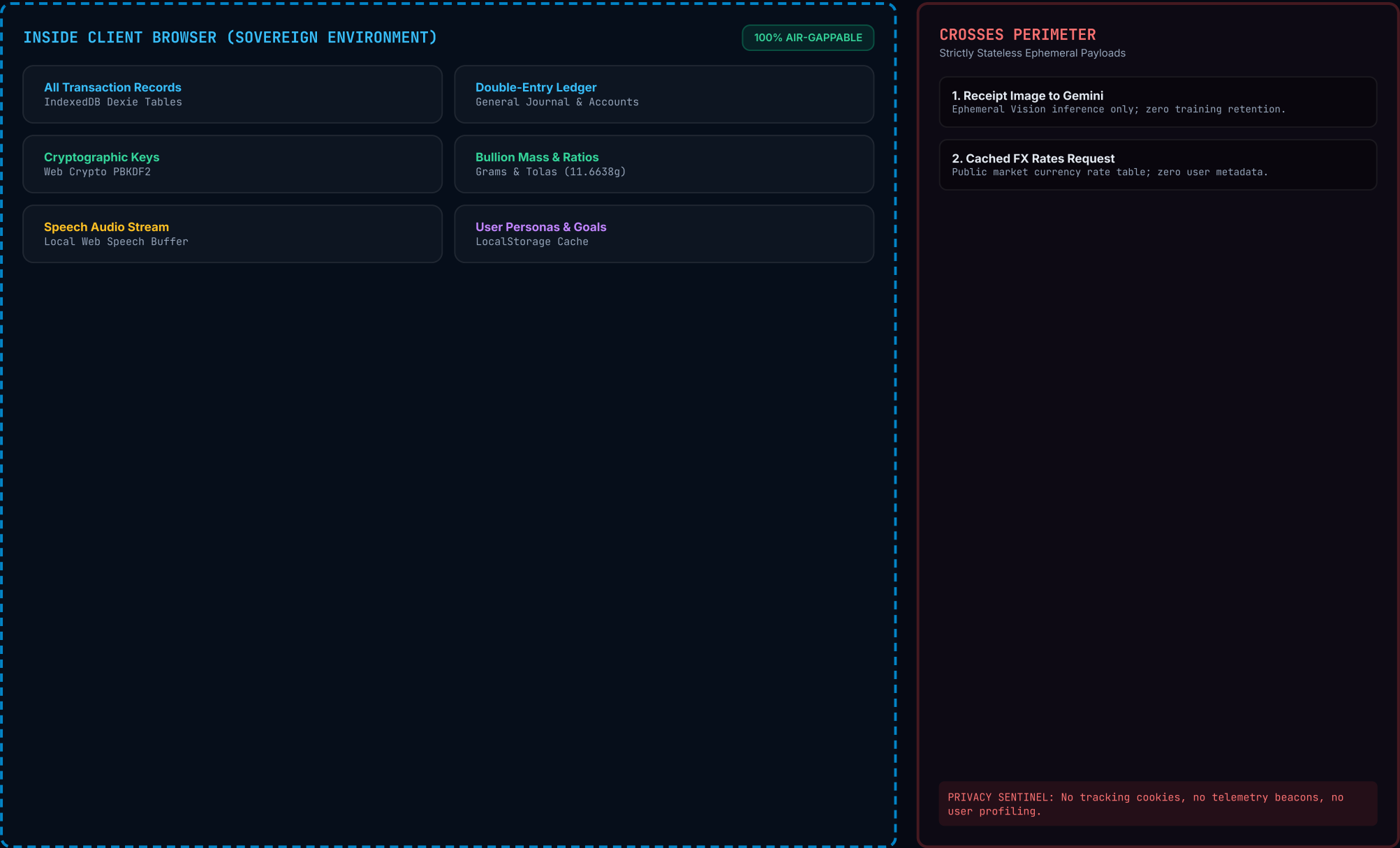
FIG. 20 – STRICT TRUST BOUNDARY SEPARATION
