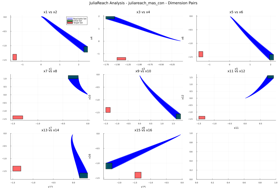
(c) Result from Set-Propagation method (JuliaReach) for benchmark MAS-CON_UNR_SAF_1.
