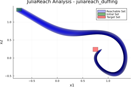
(c) Result from Set-Propagation method (JuliaReach) for benchmark DUFF_REA_BOX.
