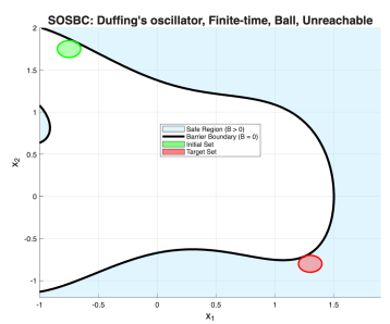
(c) Result from Barrier Certificate method (SOSTOOLS) for benchmark DUFF_UNR_CVX_LS.
