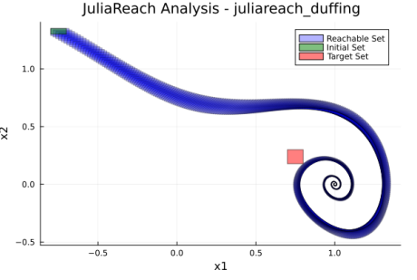
(c) Result from Set-Propagation method (JuliaReach) for benchmark DUFF_UNR_BOX.
