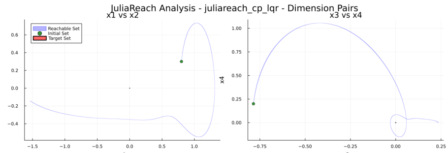
(b) Result from Set-Propagation method (JuliaReach) for benchmark CP-LQR_REA_CVG. ( Unsound Result )
