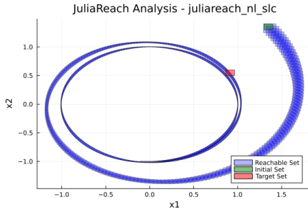
(c) Result from Set-Propagation method (JuliaReach) for benchmark NL-SLC_REA_BOX.
