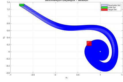
(b) Result from Set-Propagation method (CORA) for benchmark DUFF_UNR_BOX.
