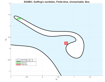
(e) Result from Barrier Certificate method (SOSTOOLS) for benchmark DUFF_UNR_BOX.
