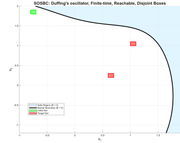
(d) Result from Barrier Certificate method (SOSTOOLS) for benchmark DUFF_REA_DSJT_BOX ( Infeasible Solution ).
