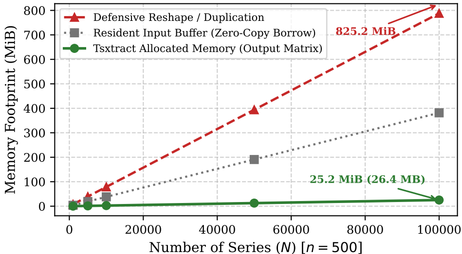
Memory Allocation during Feature Extraction
