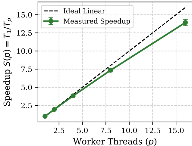
Parallel Speedup (16 Threads)
