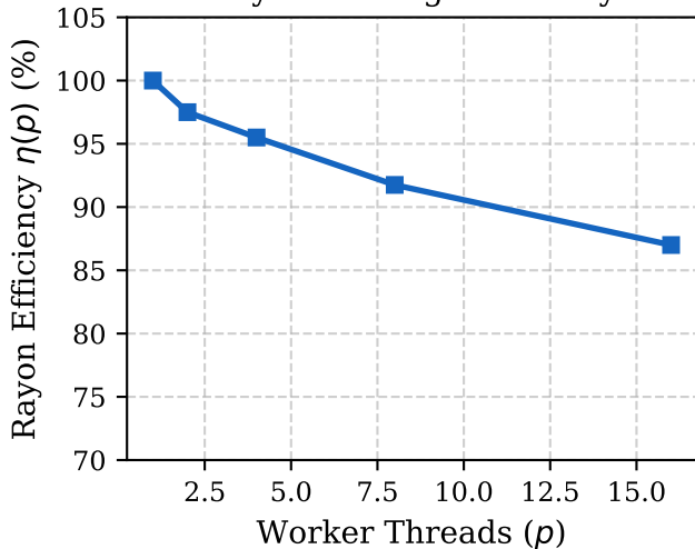
Rayon Scaling Efficiency
