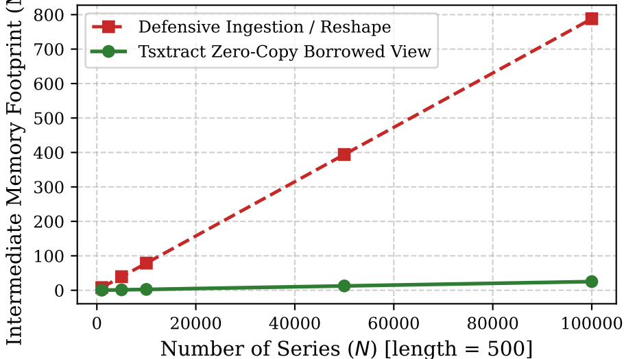
Memory Footprint During Feature Extraction
