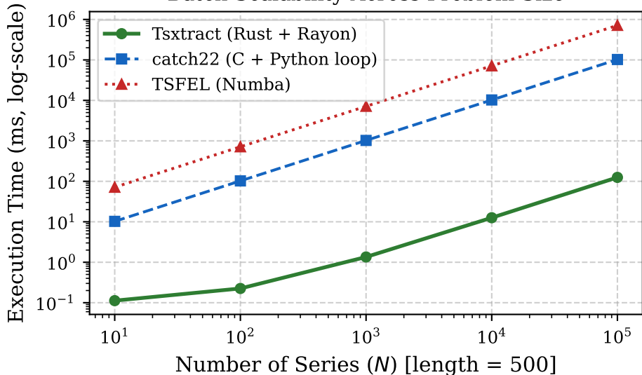
Batch Scalability Across Problem Size
