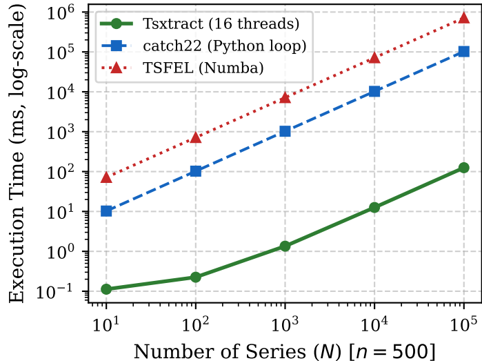
(a) Batch Scaling across N
